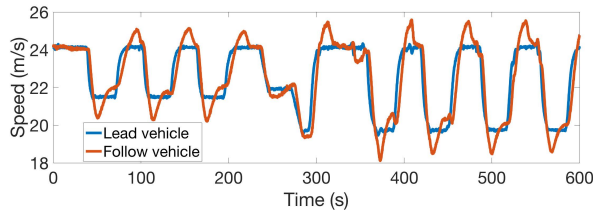
Figure 1: Sample data from car following experiment showing lead vehicle executing pre-determined speed profile and test vehicle following under ACC.
